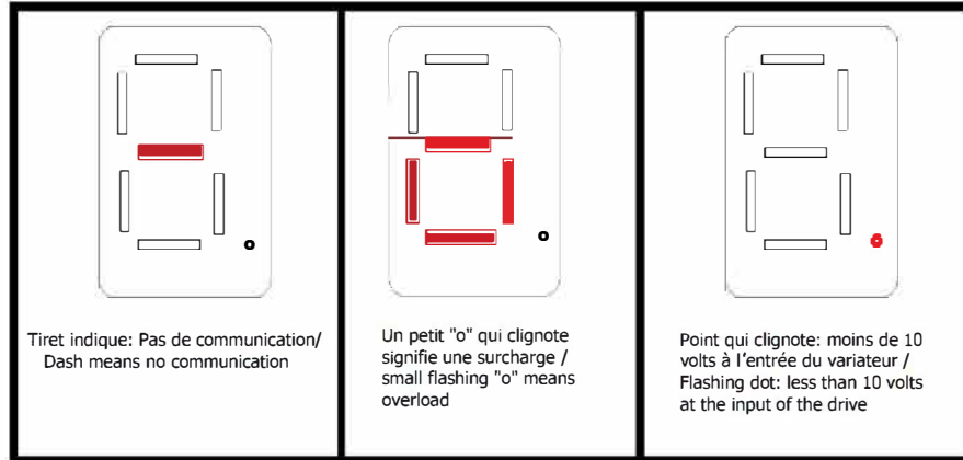
HABITACLE / IN-CAB
